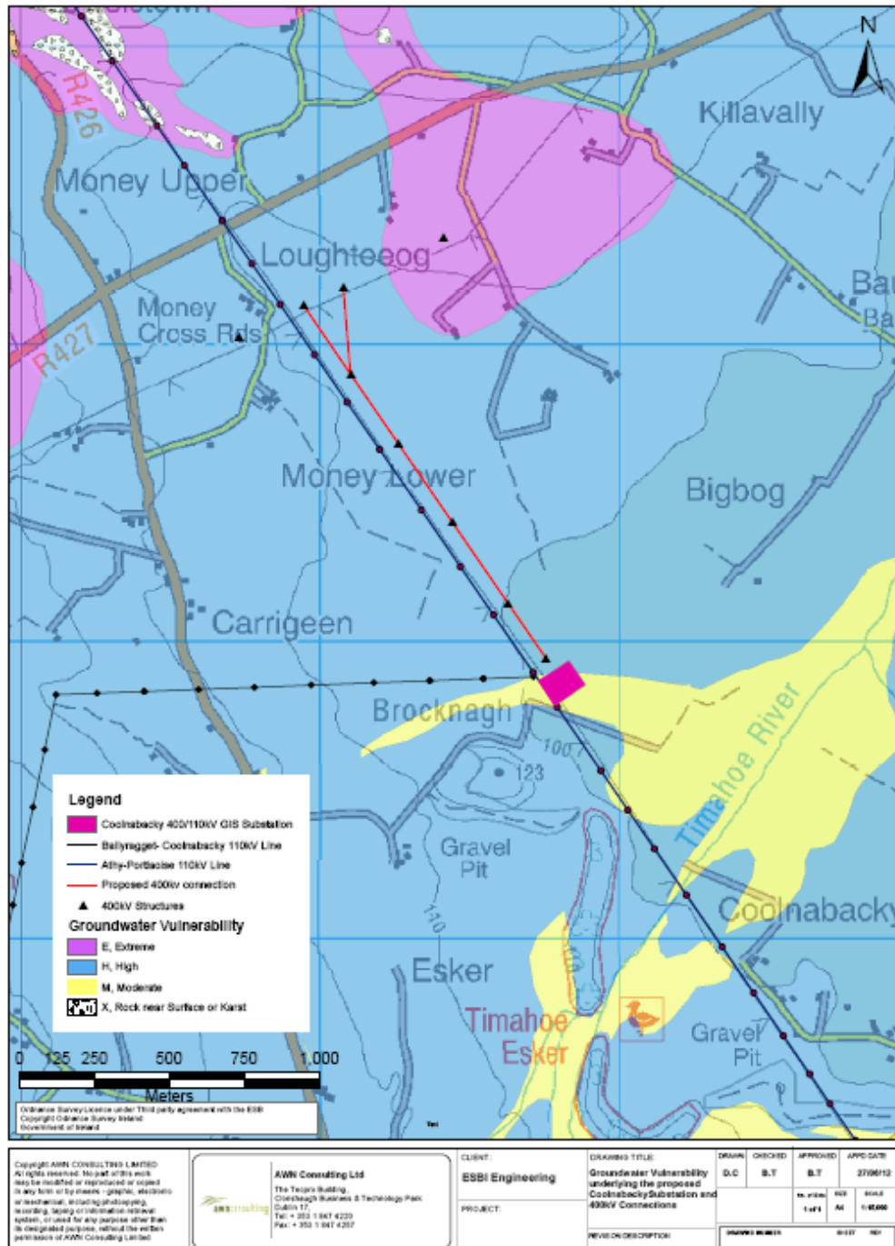
Figure 2.7 Groundwater Vulnerability underlying the proposed Coolnabacky Substation
