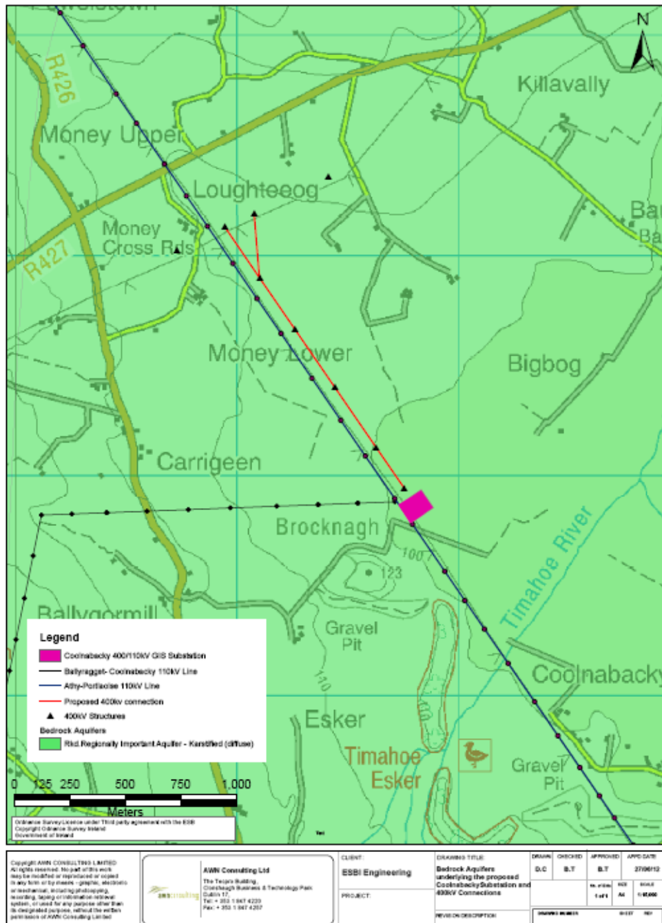
Figure 2.5 Bedrock Aquifers underlying the proposed Coolnabackey Substation
