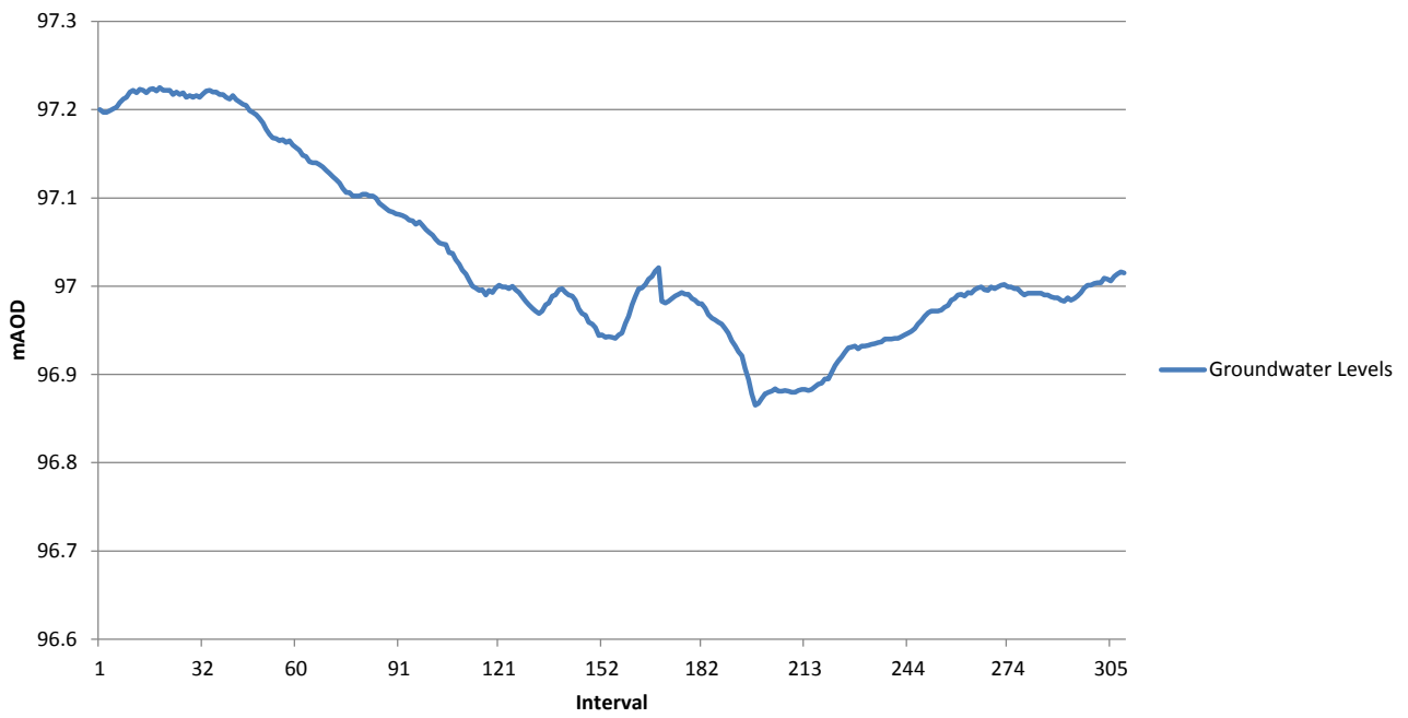
BH3 Groundwater Levels
