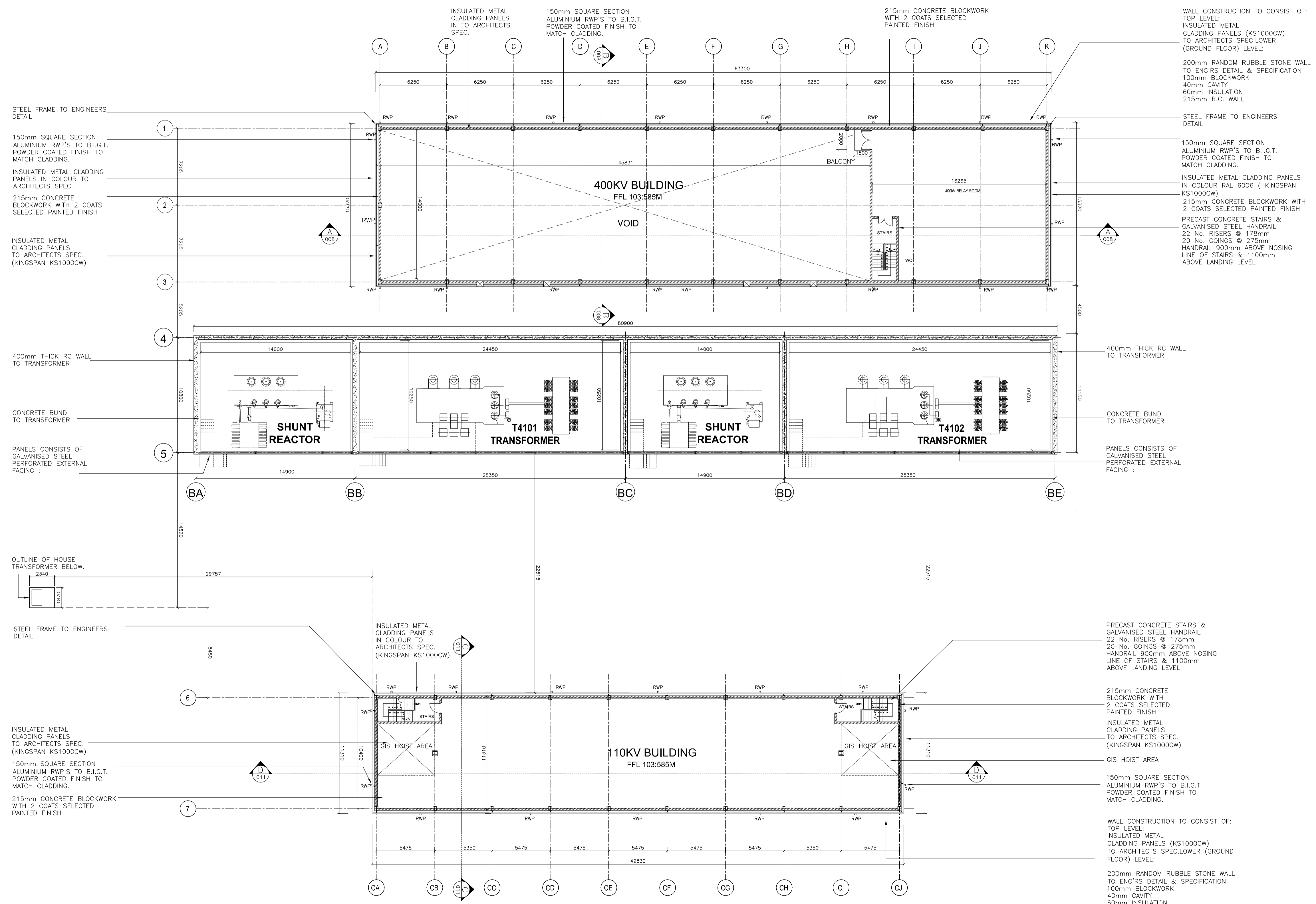
FIRST FLOOR PLANS SCALE 1:200
